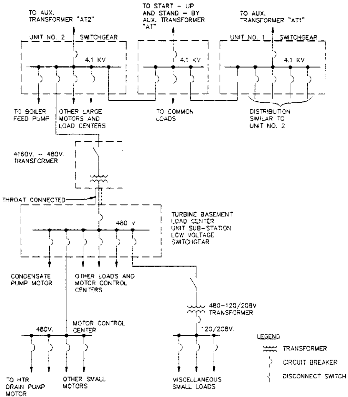
Figure 4 One line diagram, typical station service power systems
